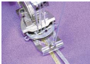
Cording foot Baby Lock Exclusive
